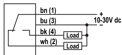
PNP (Current Sourcing) Models
