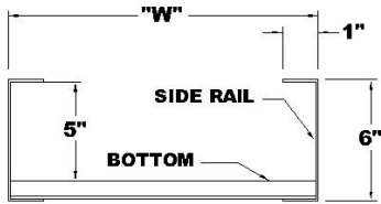
TRAY CROSS SECTION
