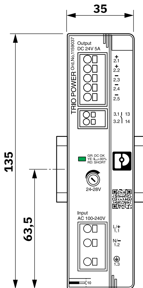
Dimensional drawing
