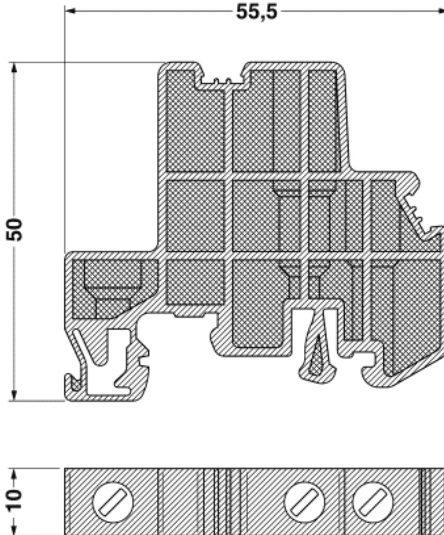
Dimensional drawing
