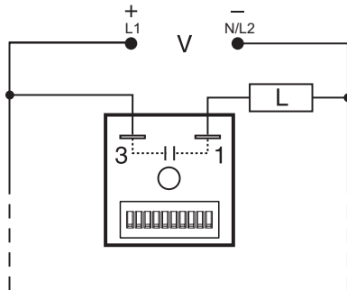
Load may be connected to terminal 3 or 1. TDU has DIP switch adjustment; KSDU is fixed.
