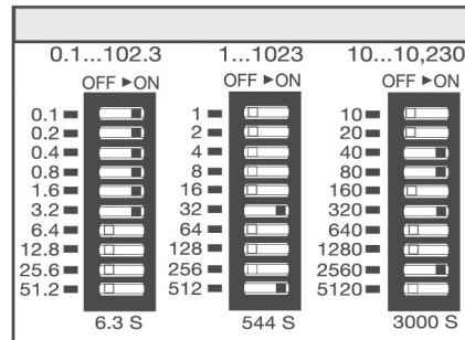
Load may be connected to terminal 3 or 1. TDU has DIP switch adjustment; KSDU is fixed.
