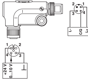
Connection diagram
