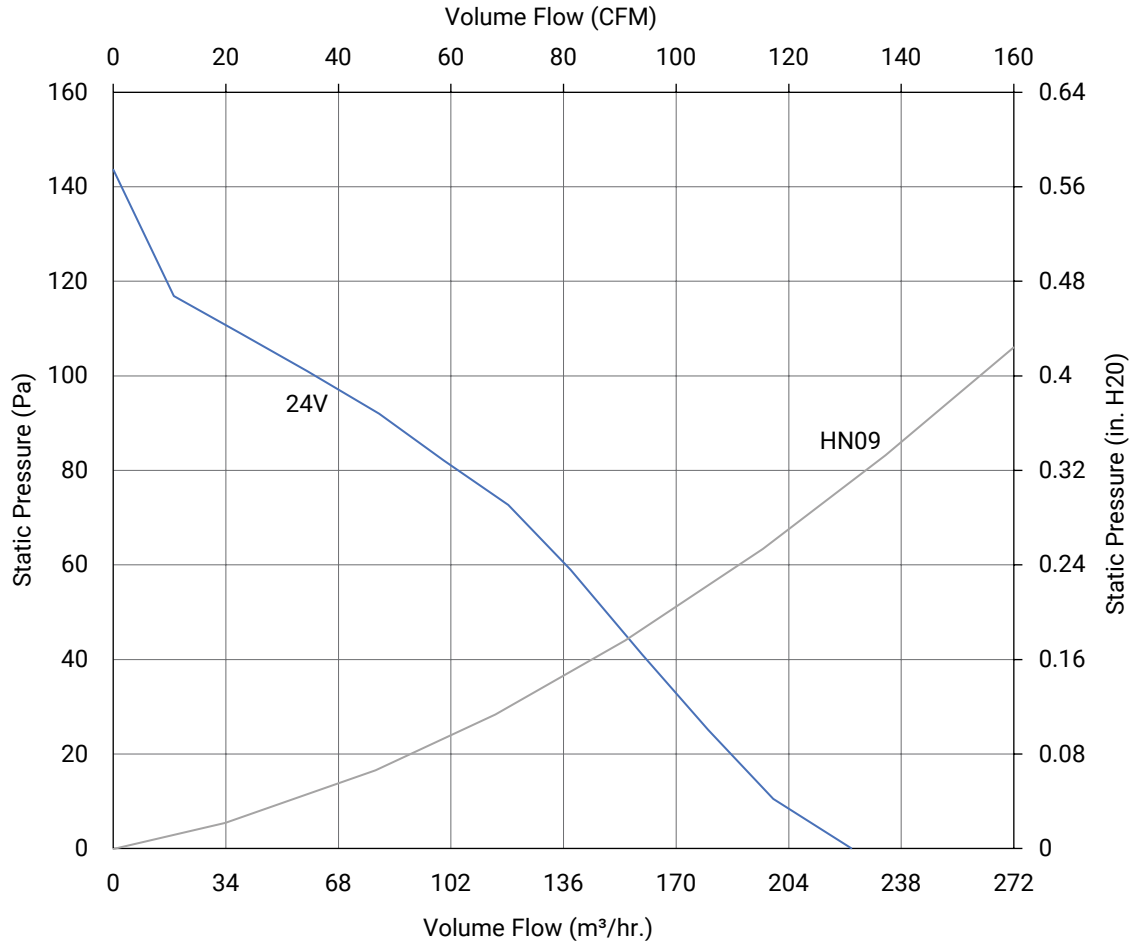
HN09 Capacity Curve, IP55
