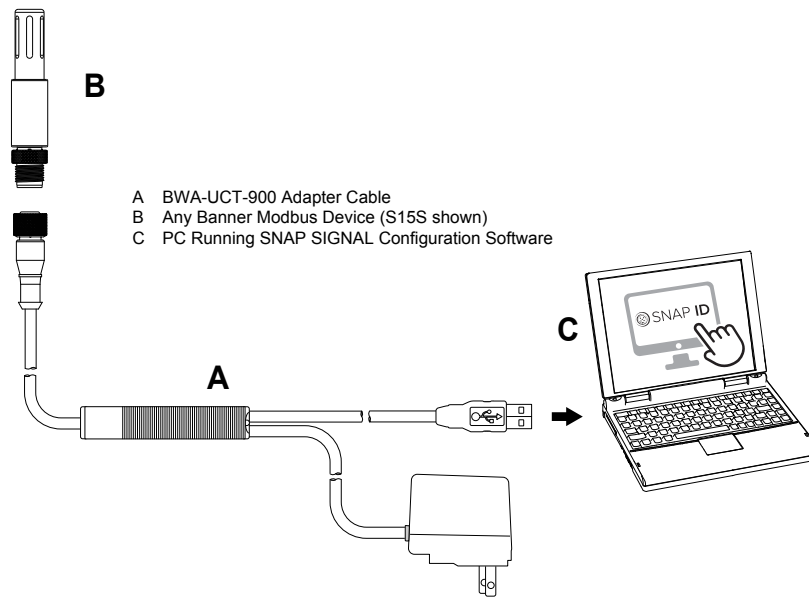
Figure 1. Banner Modbus Device Connection
