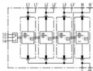
Basic circuit diagram DVA CSP 3P 100 FM
