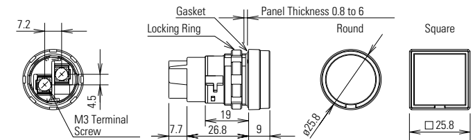
ø22 EB3P-LLW1/EB3P-LLW2/EB3P-LLW3 Terminal cover attached.
