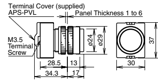
ø22 EB3P-LHW1/EB3P-LHW2/EB3P-LHW4 Terminal cover attached.
