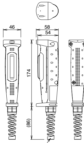
Cable Gland (supplied with grip switch) Type No.: SKINTOP BS-M20 x 1.5 (LAPP)
