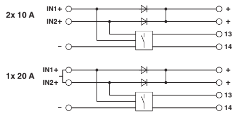
Block diagram
